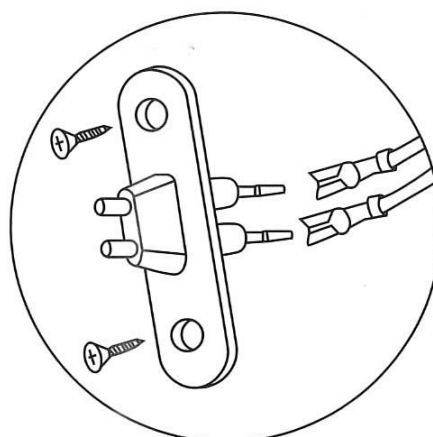
SLIDE DOOR CONTACT SWITCH MOUNTING DIAGRAM
